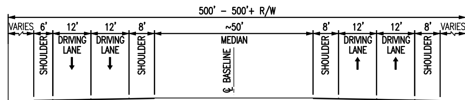
TYPICAL SECTION 1 RABBIT ROAD TO NORTH OF MERGE
