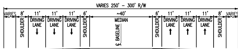
TYPICAL SECTION 3 SOUTH OF SAWMILL ROAD TO ST. MICHAELS DRIVE RAMPS
