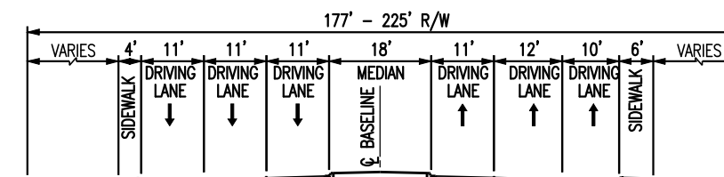
TYPICAL SECTION 8 SOUTH OF CAMINO DE LAS CRUCITAS TO NORTH OF ALAMO DR.
