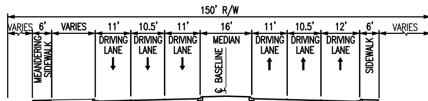
TYPICAL SECTION 4 WEST SAN MATEO ROAD TO WEST CORDOVA ROAD
