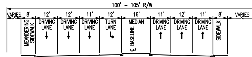
TYPICAL SECTION 5 WEST CORDOVA ROAD TO CERRILLOS ROAD
