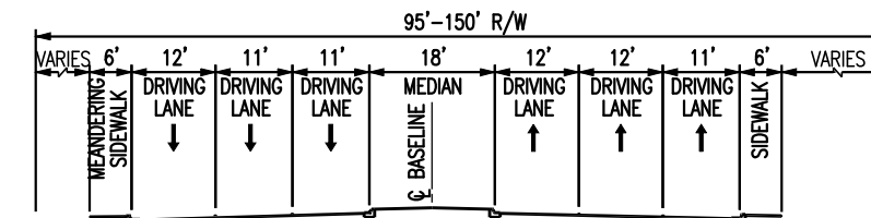
TYPICAL SECTION 7 NORTH OF MERCER ST. TO SOUTH OF CAMINO DE LAS CRUCITAS
